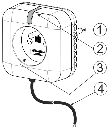
Fig. 1: 1 – UniSchuko plug; 2 – function button/indicator; 3 – French socket, 4 – potential-free switched output cable
