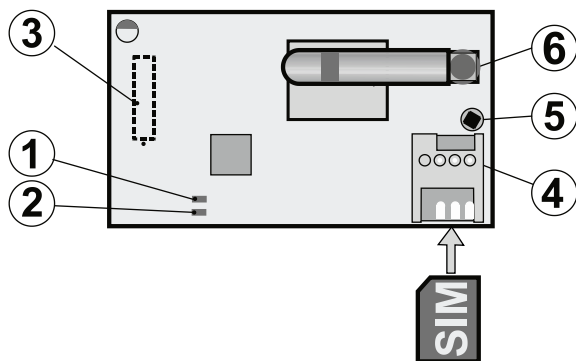
Fig. 1: JA-191Y Communicator
