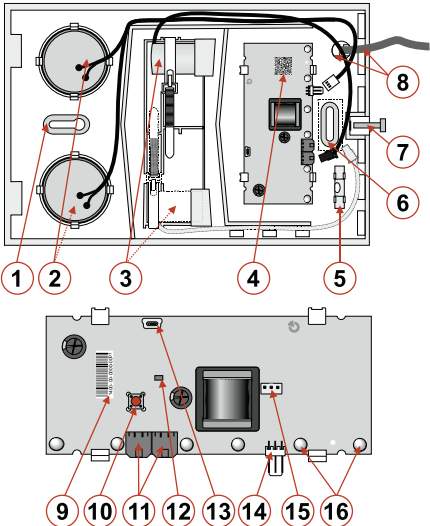
Figure 1: Description of internal parts of the product
