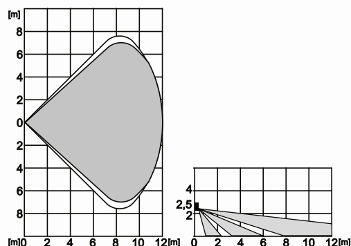
Fig 2: detection characteristic
