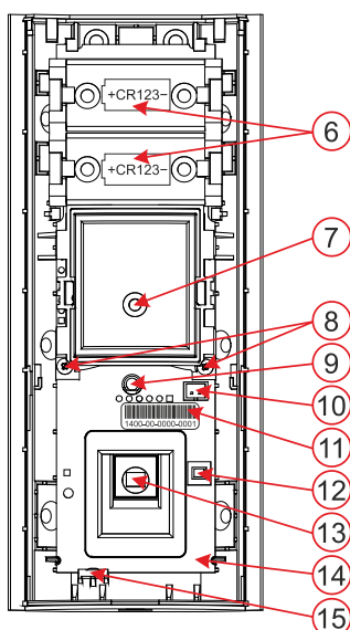
Figure 2: Description of internal parts of the product
