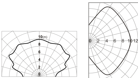
Figure 4: Detection characteristics of the GBS sensor.
