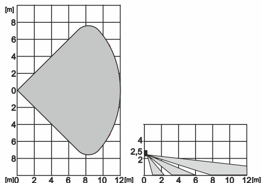
Figure 3: Detection characteristics of PIR detector
