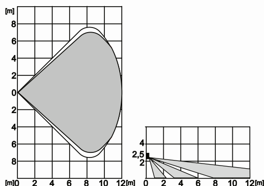
Figure 3: Coverage characteristics
