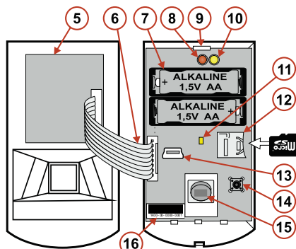
Figure: 5 – Camera module; 6 – connection cable; 7 – batteries; 8 – red LED indicator; 9 – PCB tab; 10 – yellow LED; 11 – yellow LED indicator of Micro SD card; 12 – Micro SD memory card; 13 – mini USB connector; 14 – tamper contact; 15 – PIR sensor; 16 – production code.
