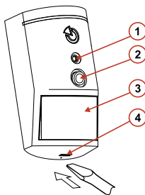
Figure: 1 – flash for illumination; 2 – camera lens; 3 – PIR detector lens; 4 – cover tab;
