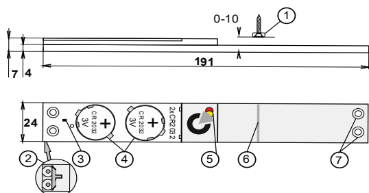
Figure: 1 – magnet; 2 – tear-removal mechanism for removal detection (on the back side of the detector); 3 – cover tamper sensor; 4 – batteries (2x CR 2032); 5 – hidden LED indicators (under the logo); 6 – adjustment line; 7 – fixing holes
