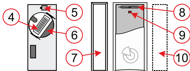
Figure 3: 4 – serial number; 5 – tamper contact; 6 – battery; 7 – permanent magnet; 8 – magnetic sensor; 9 – red detector activation indicator; 10 – alternative placement of the permanent magnet
