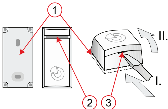
Figure 1: 1 – separation plate; 2 – red activation indicator; 3 – cover tab
