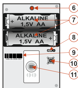
Figure 2: 6 – LED indicator; 7 – batteries; 8 – immunity setting jumper; 9 – serial number; 10 – tamper contact; 11 – PIR sensor
