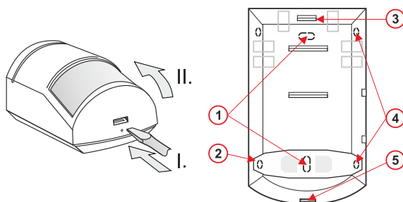
Figure 1: 1 – holes for installing on a flat wall; 2, 4 – holes for installing at an angle (in a corner); 3 – PCB latch; 5 – cover latch
