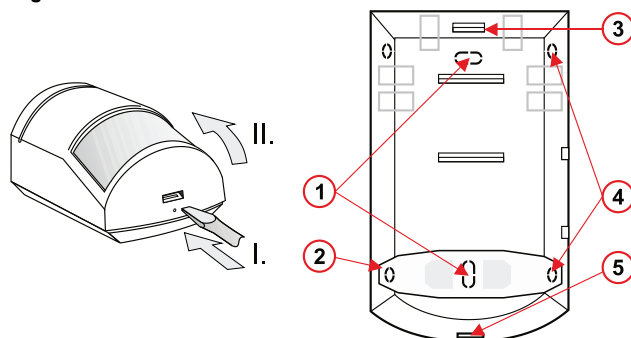
Figure 1.: 1 – holes for installing on a flat wall; 2, 4 – holes for installing at an angle (in a corner); 3 – PCB tab; 5 – cover tab
