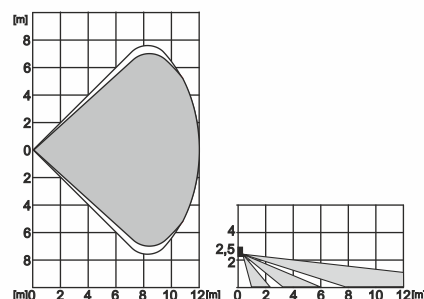
Fig. 2: Detection characteristics
