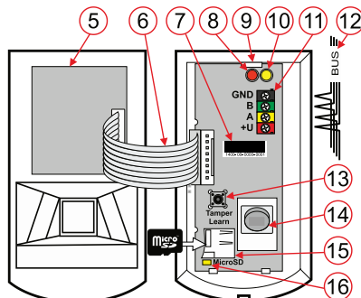
Figure: 5 – Camera module; 6 – connecting cable; 7 – production code; 8 – red LED indicator; 9 – PCB tab; 10 – yellow LED indicator; 11 – BUS terminals; 12 – BUS cable; 13 – tamper contact; 14 – PIR sensor; 15 – micro SD memory card; 16 – yellow LED micro SD card indicator
