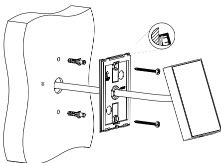
Fig. 2: Card reader installation
