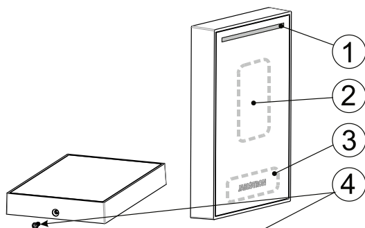
Fig. 1: 1 – LED indicator, 2 – 125 kHz reading zone, 3 – 13.56 MHz reading zone, 4 – locking screw
