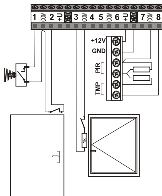
Figure: Loop connection example
