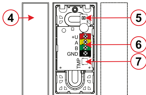
Figure 2: Description of internal parts of the detector: 4 – permanent magnet; 5 – LED indicators; 6 – bus terminals; 7 – tamper
