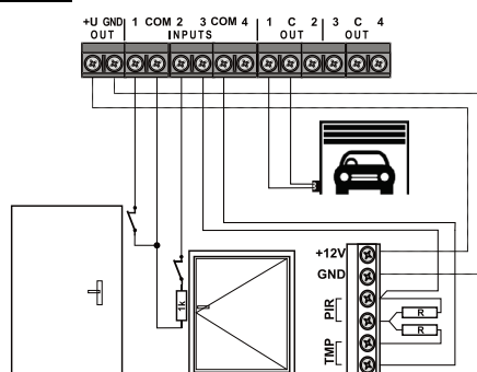
Figure 1: Wiring example
