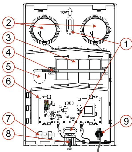
Figure 1: Description of internal parts of the product
