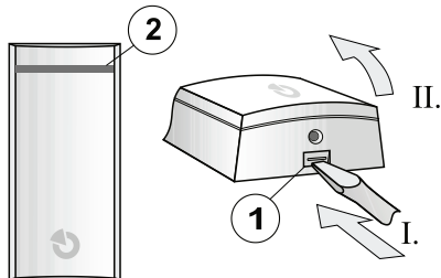
Figure 1: 1 – cover tab; 2 – LED indicator
