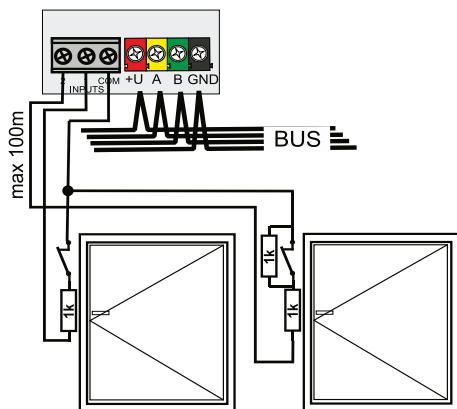
Figure 3: Loop balancing
