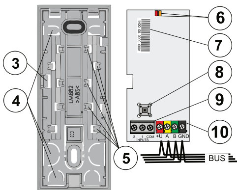
Figure 2: 3 – PCB tab; 4 – cut-out holes; 5 – fixing clips for cables coming from the top cut-out holes; 6 – red and yellow LED indicator; 7 – production code; 8 – tamper sensor; 9 – magnetic contact terminal; 10 – bus terminal
