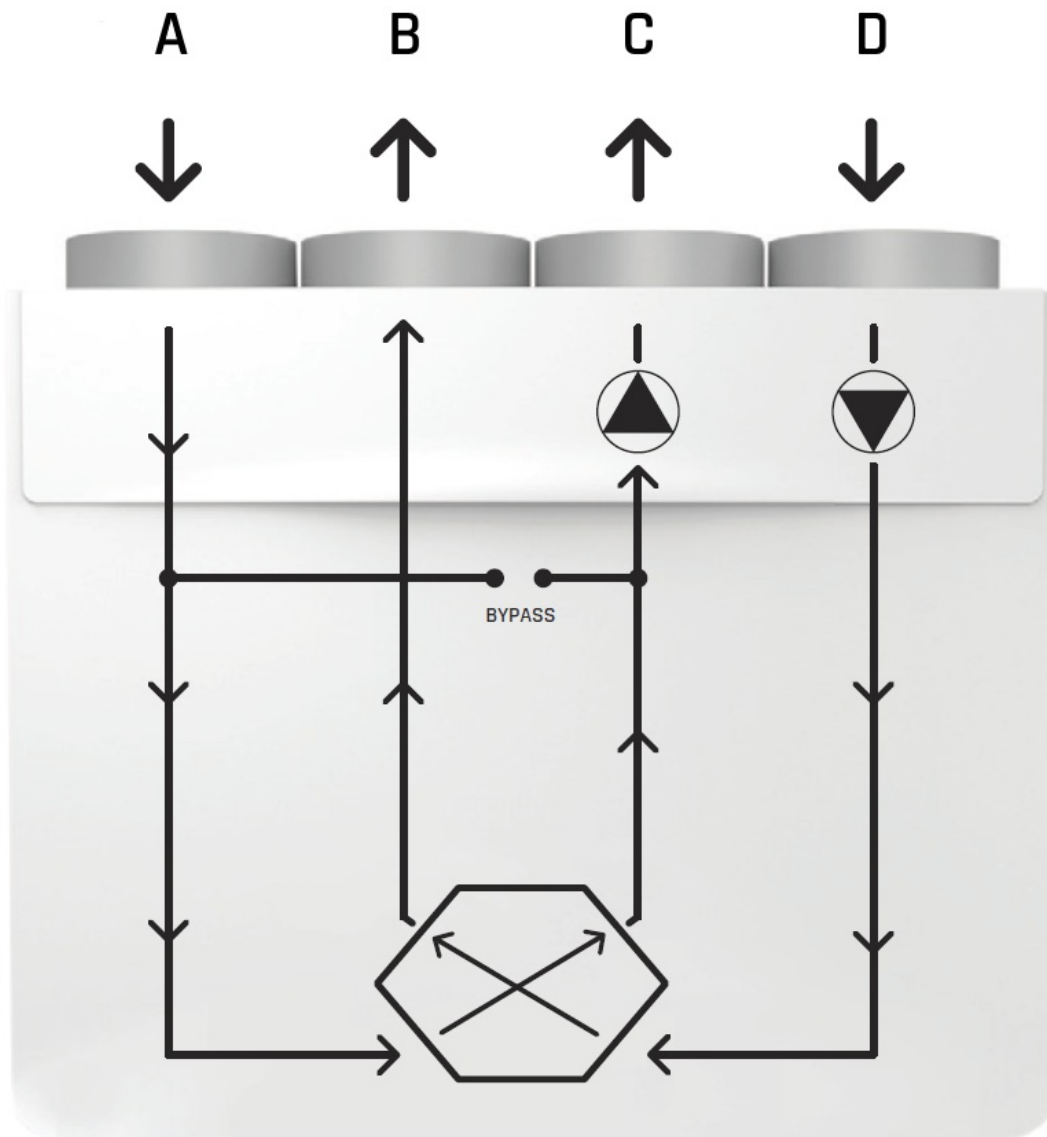
Figure 2 – Heat recovery principle
