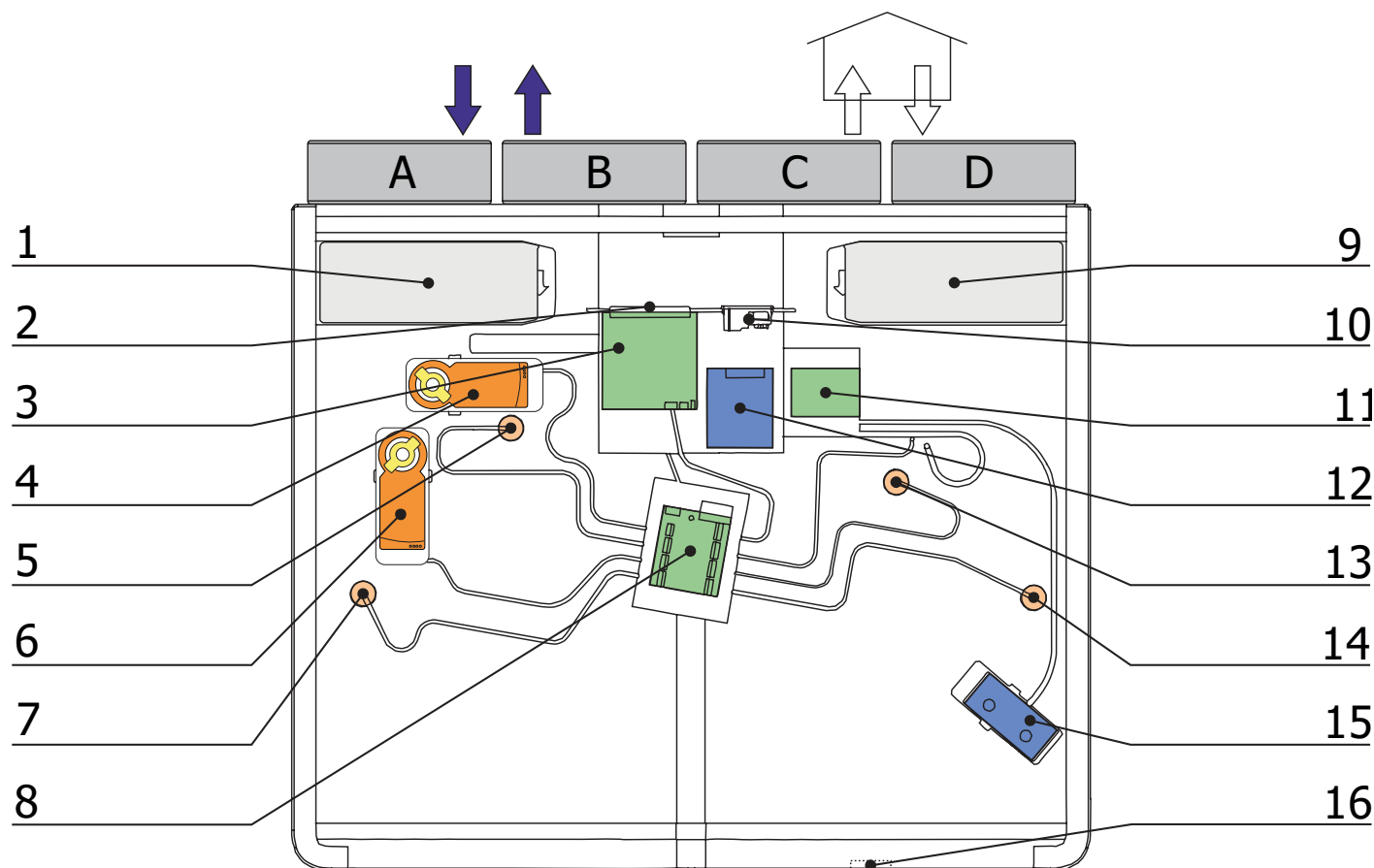
Figure 3 – Unit structure
